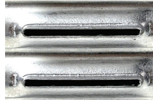
OSC Ribbed Header With Expanded Tube Openings
