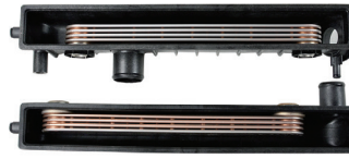
OSC Ribbed Header With Expanded Tube Openings
