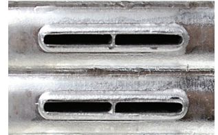
Competitor: Ribbed Header with "B-Tube" Design
