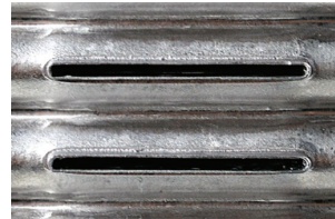
OSC Ribbed Header
